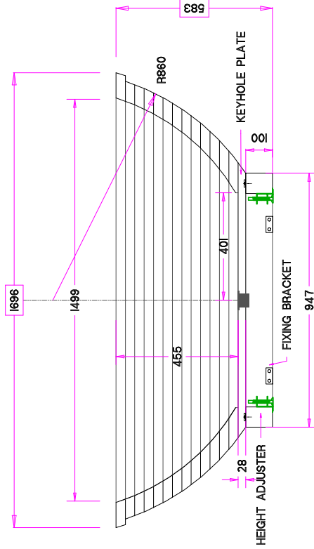
SECTION THROUGH BATH NTS
